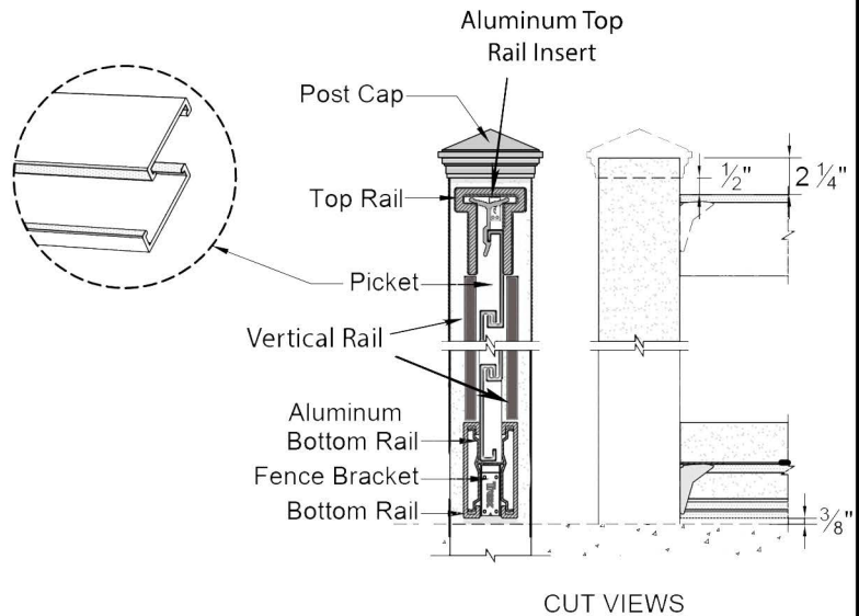
CUT VIEWS
