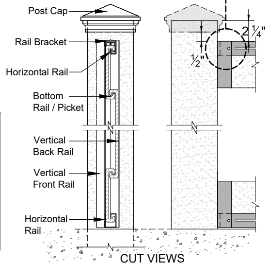
CUT VIEWS
